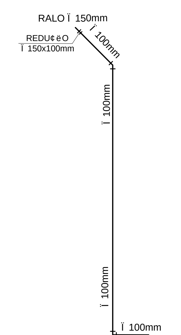
DETALHE 2 TUBO DE QUEDA APs.: 1,2,3,4,5,6,8, 9,11,14,15,16,18, 19,31,32,33,34,37, 38,39,40 e 42
