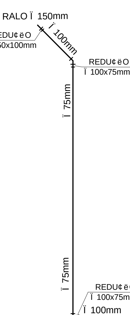
DETALHE 4 TUBO DE QUEDA APs.: 20,23,24,25,27, 28,29,30,35,36,
